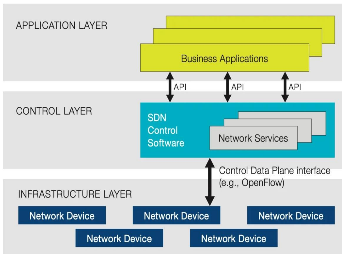
Fig 2: SDN Architecture
