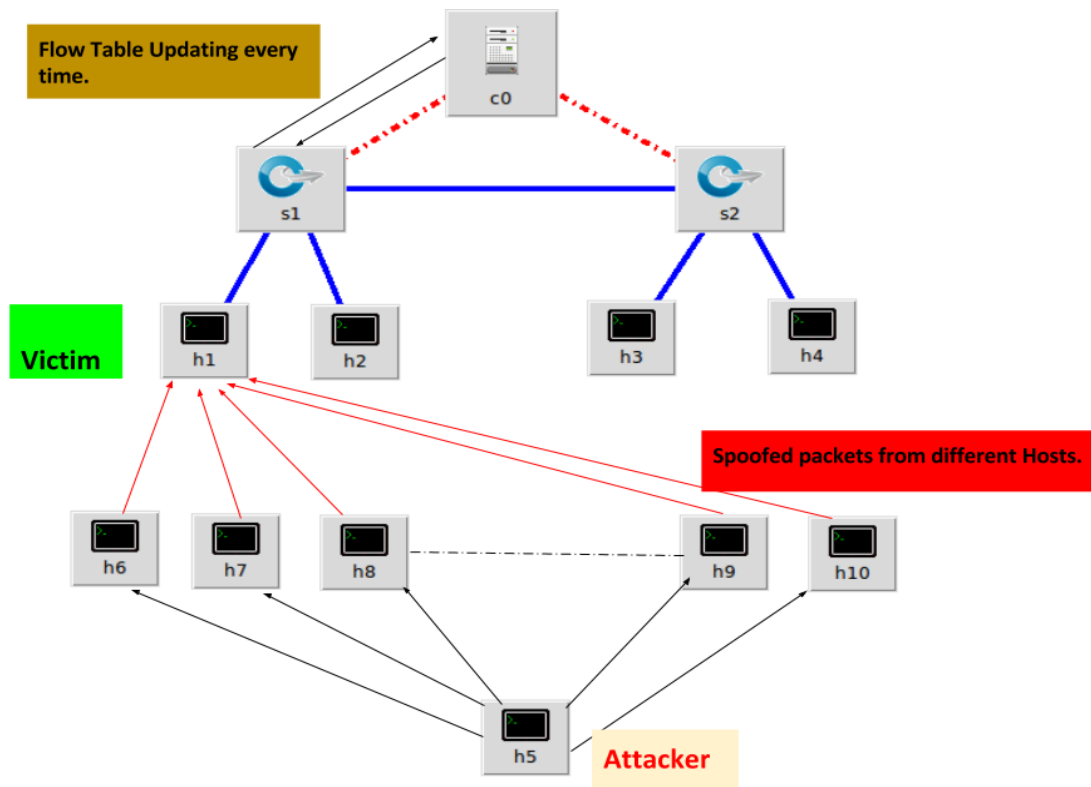
Fig 3: DDoS attack on SDN
