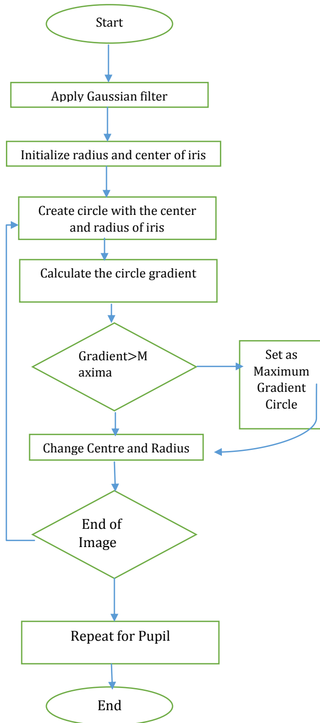
Fig 1.Flow Chart of Daugman Algorithm
