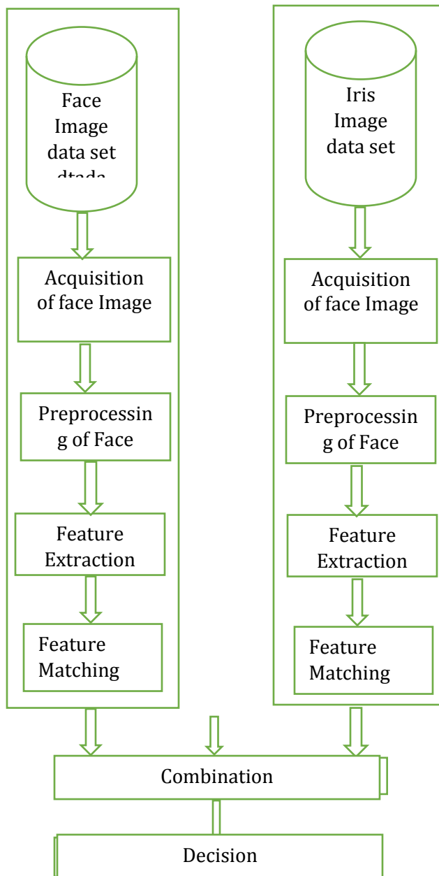
Fig. 4. Flowchart of Face and Iris recognition using Combined PCA-Daugman Method
