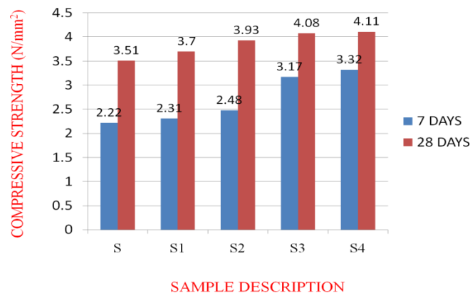
COMPARISON OF COMPRESSIVE STRENGTH RESULTS
