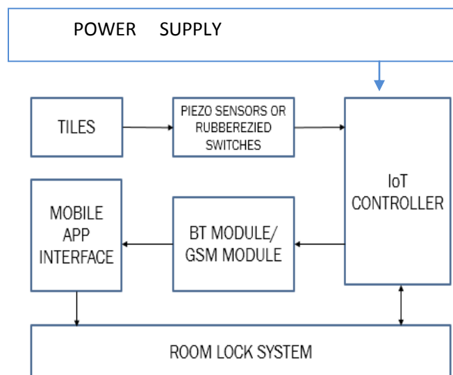
Figure 1: Block diagram
