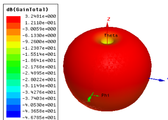
Fig.6. Simulated 3D polar plot of DRA
