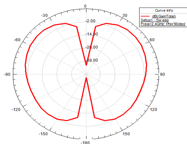
(b) H-plane radiation pattern at 2.4GHz
