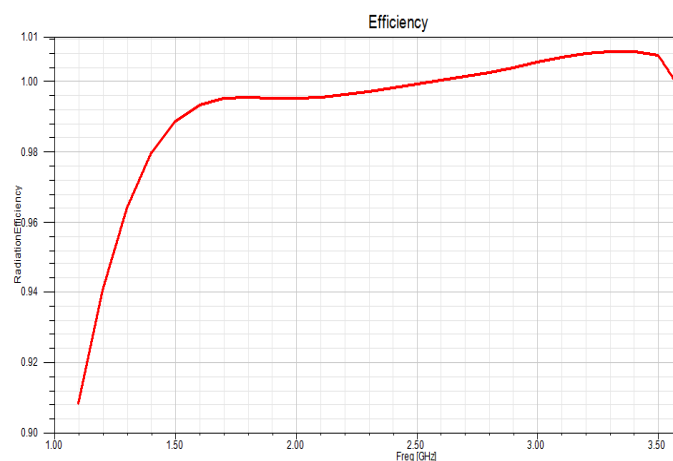
Fig.5. Efficiency Curve of DRA
