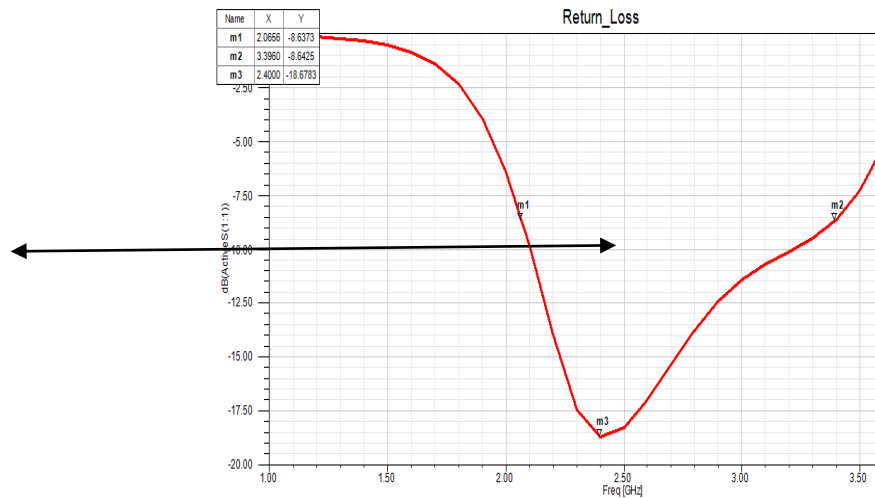
Fig.3. Simulated Return Loss of DRA
