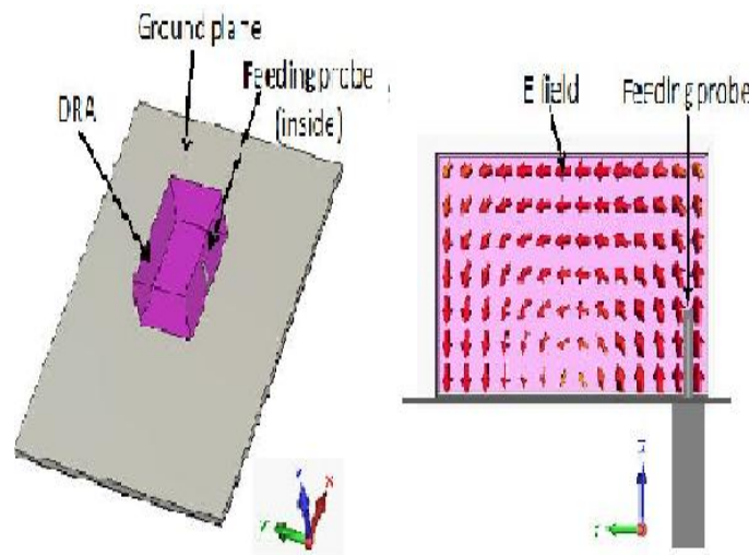
Fig.1. Rectangular Dielectric Resonator Antenna and Field Pattern [4]
