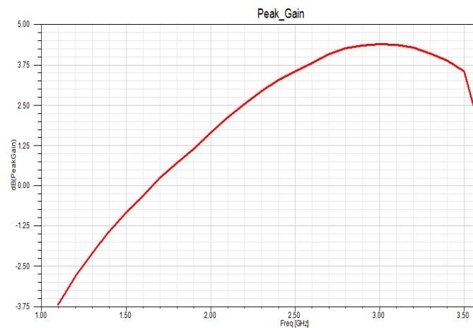
Fig.4. Simulated peak gain of DRA
