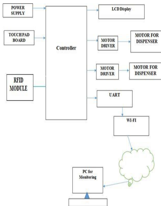
Figure1: Automatic vending machine for medicines
