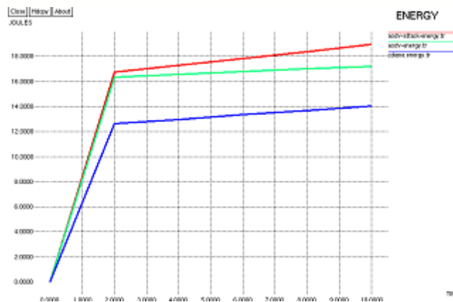
Fig.3. Variation of energy consumption with time
