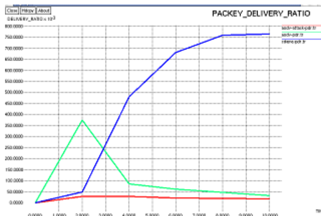
Fig.2. Variation of Packet delivery Ratio with Time
