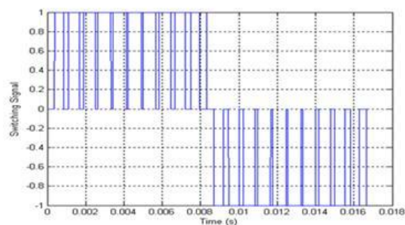
Figure 2: switching signal
