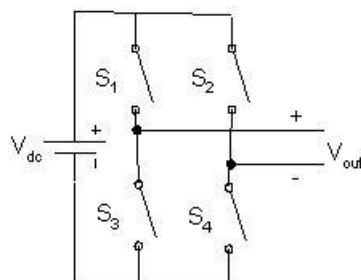
Figure 5: Two-phase capacitor-clamped multilevel converter
