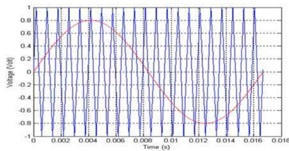
Figure 1: Sine-triangle PWM control sinusoidal reference signal and triangle carrier signal
