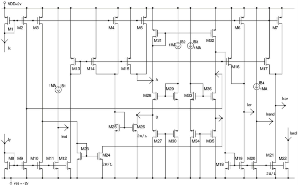
Figure 1. Proposed implementation of the NOT/OR/NAND/XOR /AND digital logic functions using analog techniques.
