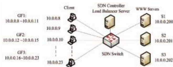
Figure 4. Structural model experiment system network configuration
