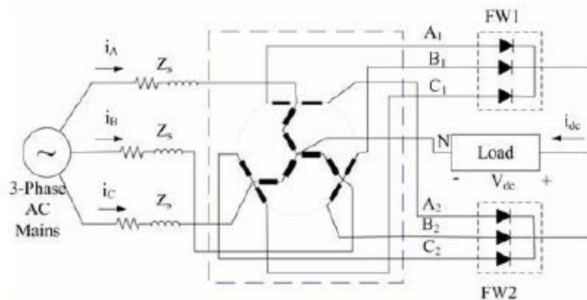
Fig. 2: Proposed zigzag autotransformer based 6-pulse full-wave AC-DC converter.
