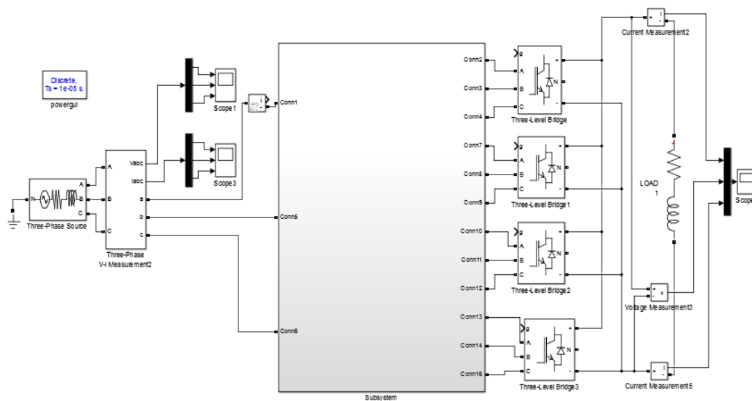
Fig.4a. MATLAB model of 24-pulse AC-DC converter
