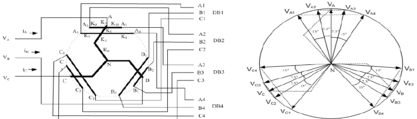
Zigzag autotransformer winding arrangement for 24-pulse AC-DC con
