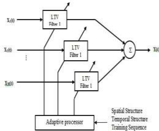
Fig.4.1 Typical Array Processing Architecture
