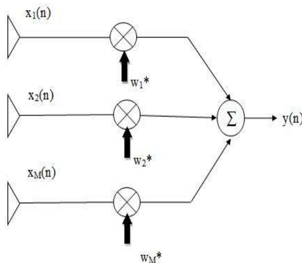
Fig. 3.2 Beam forming Operation
