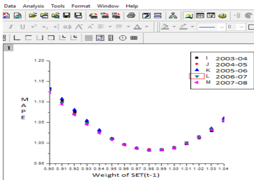
Figure 2: MAPE at different b(0) from Jan 2003 to April 2008 with two years training data scale from 0.90 to 1.04
