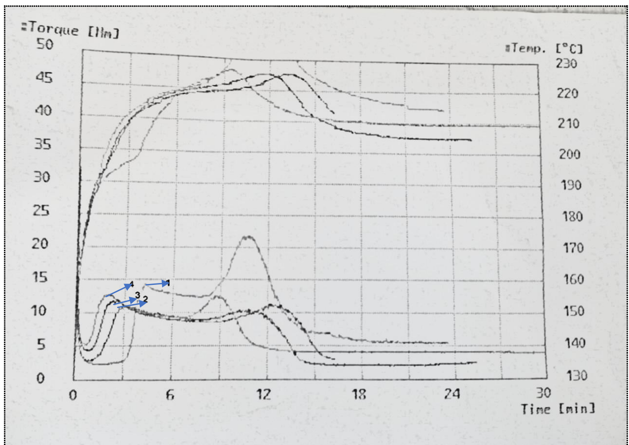
Fig.5.Content on fusion time, torque and stability time.
