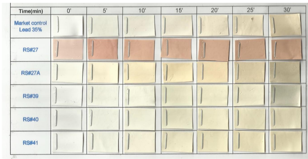
Fig. 2. Oven Stability test for stabilizers. Color changes of PVC strips at 190°C. [RS- research sample] Stabilizer containing pentaerythritol having value of 0.12g with formulation A shows good long-term stability. Colorimeter Data for above PVC strips, whiteness and yellowness index as shown in table no.6 and 7 respectively.
