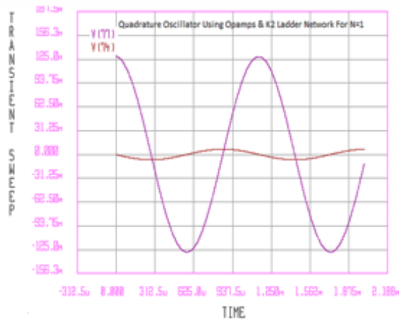
Fig. (8) Output Waveforms of Quadrature Oscillator for Control Word N=1
