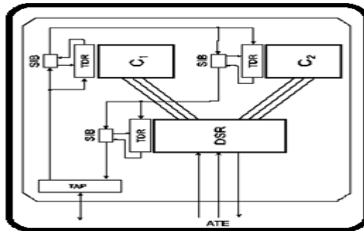
Fig.1. Transfer control data using IJTAG network
