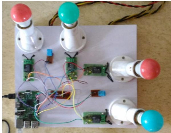
Fig.2: Experimental Setup
