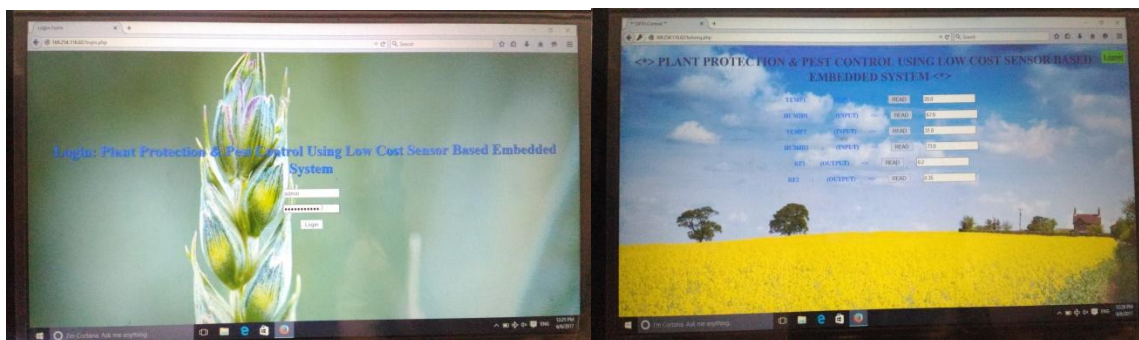
Fig.3: Webpages
