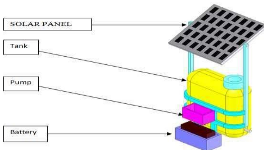
Fig.1: Layout of Solar pesticide sprayer
