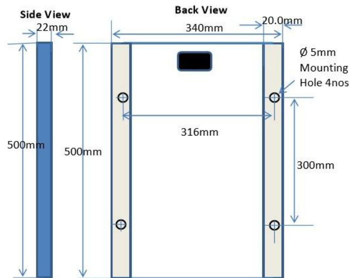
Fig.3: Photo voltaic module dimensions
