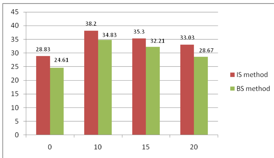
Fig. 2: Graphical representation of 28 days strength obtained for M40 mixes
