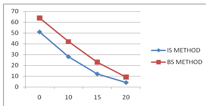
Fig..6: Graphical representation of Slump for M50 grade at varying % of alccofine
