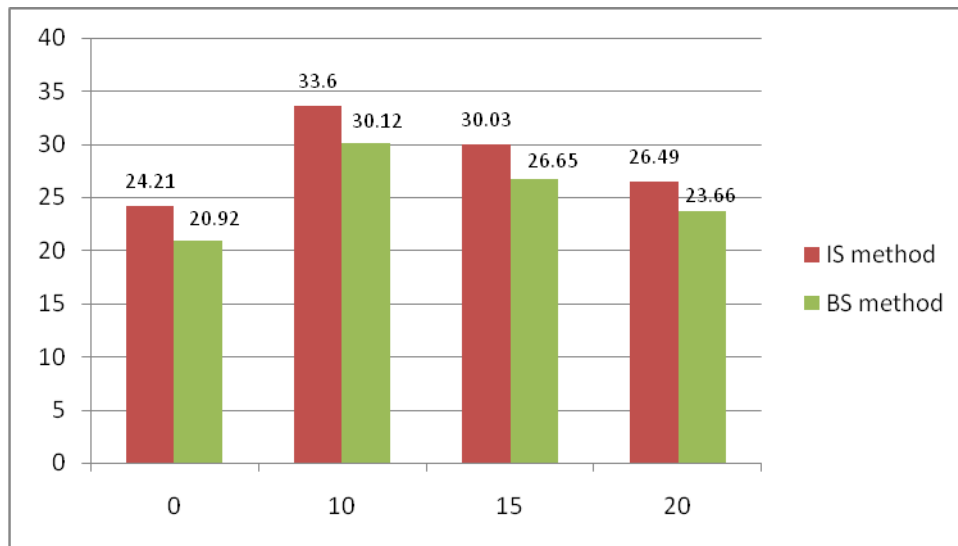
Fig. 3: Graphical representation of 7 days strength obtained for M50 mixes
