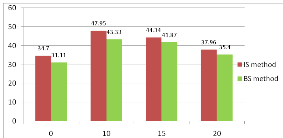
Fig. 4: Graphical representation of 28 days strength obtained for M50 mixes
