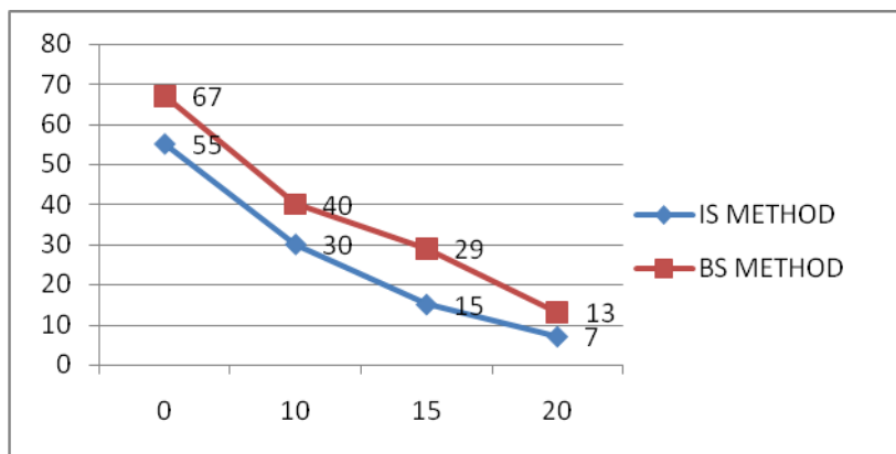
Fig.5: Graphical representation of Slump for M40 grade at varying % of alccofine
