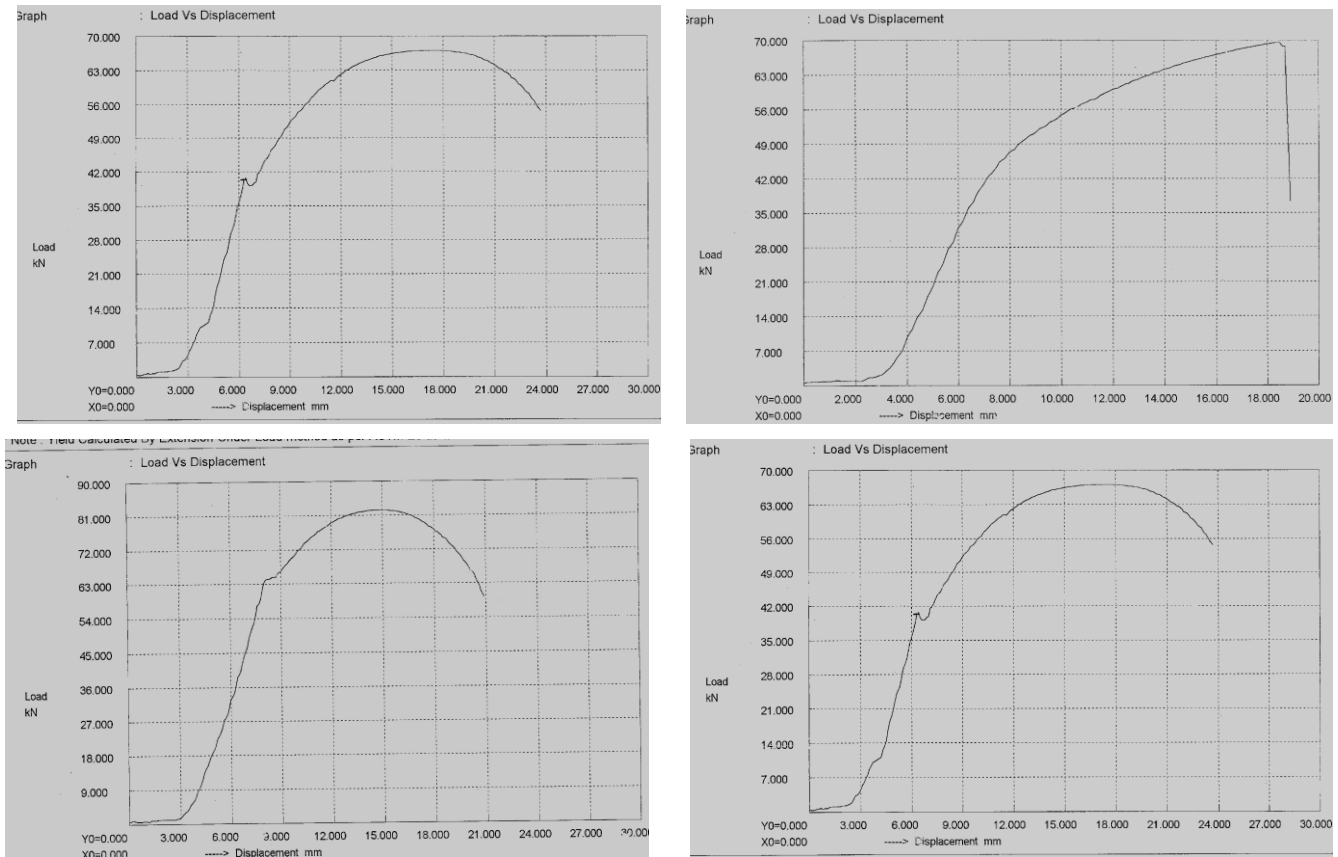
Fig. 3 Tensile Stress Graphs for (a) Sample 1 (b) Sample 2 (c) Sample 3 (d) Sample 4
