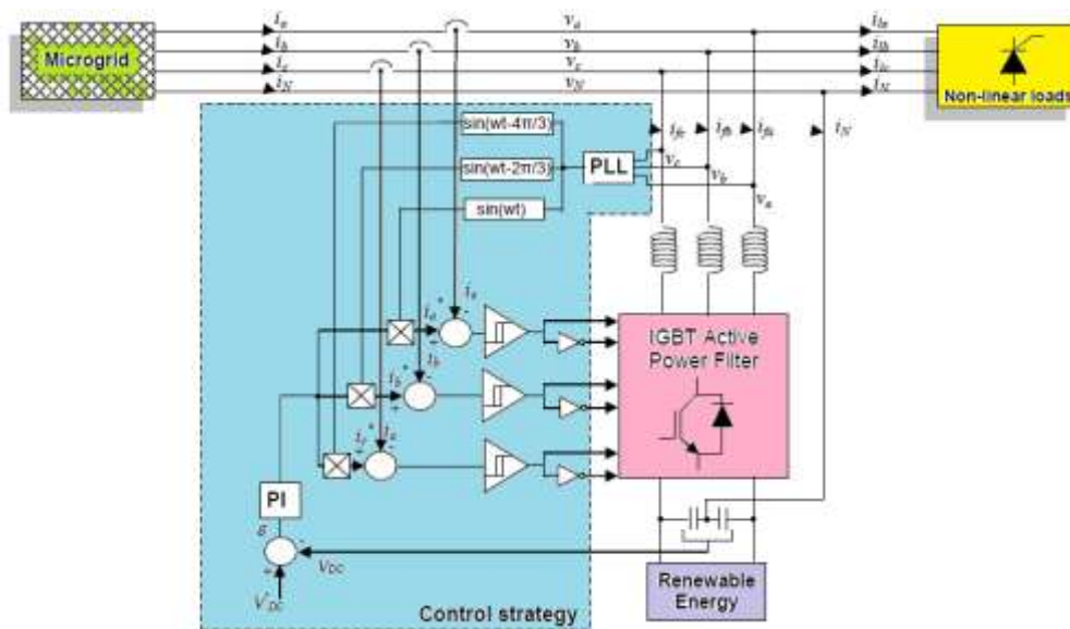
Figure 4. APC Control Strategy
