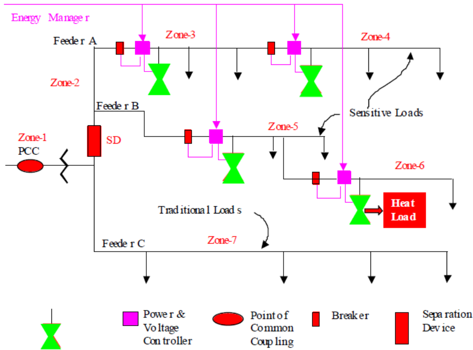
Fig.2 Microgrid Architecture
