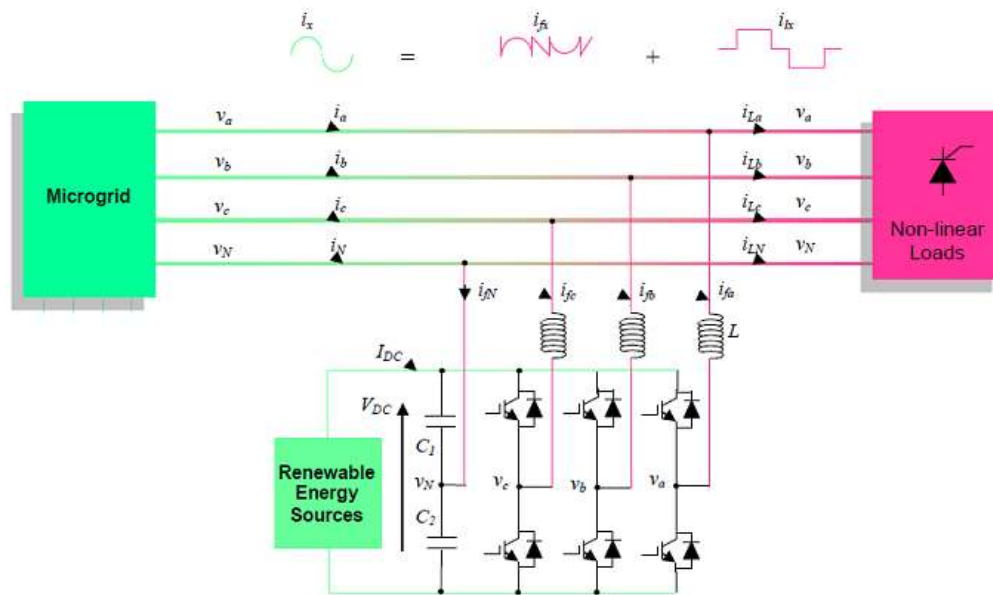
Figure 2. APC Topology
