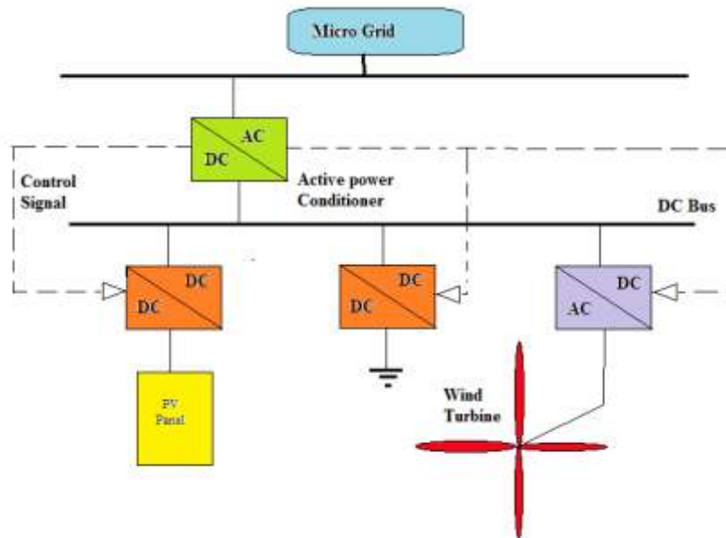
Figure 1. APC for Microgrid applications
