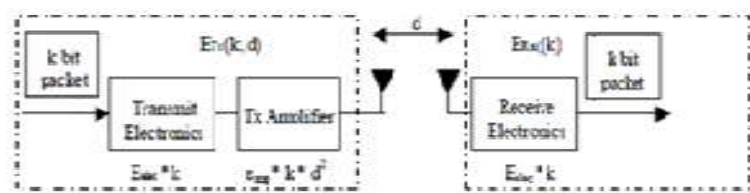
Fig.3 – Radio Energy Model [9]
