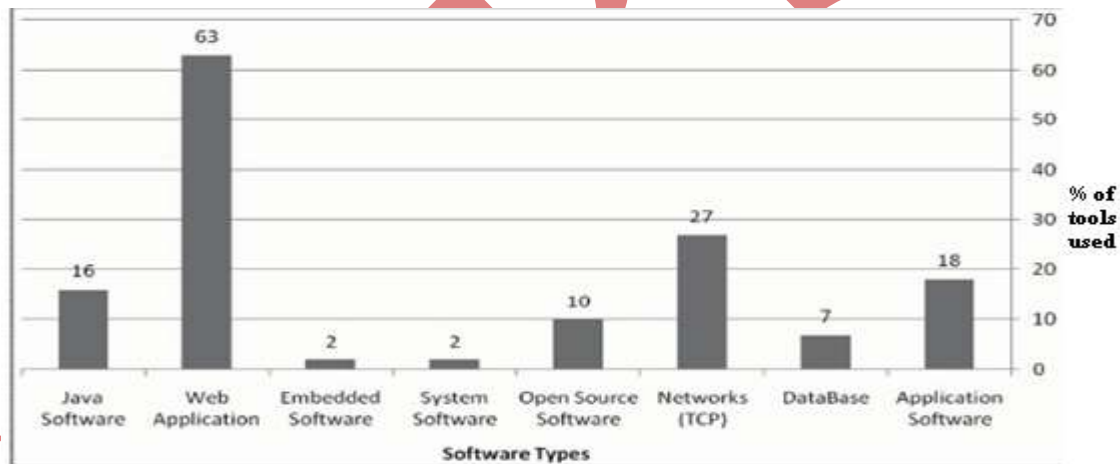
Fig. 1: Distribution of the used testing tools over the software types.
