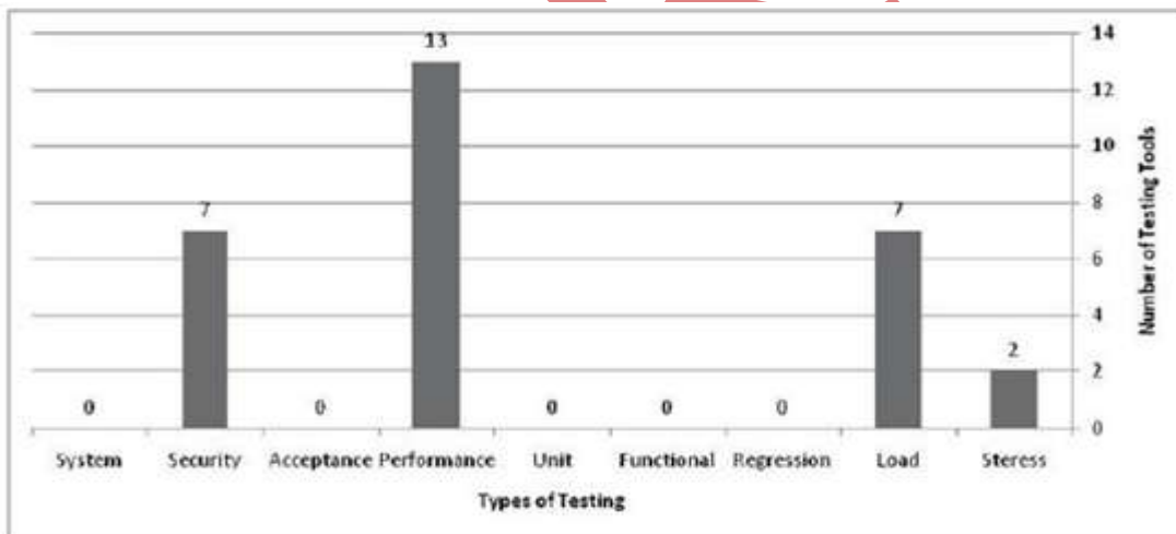
fig 3: Distribution of the testing tools for networks(TCP) over the type of testing
