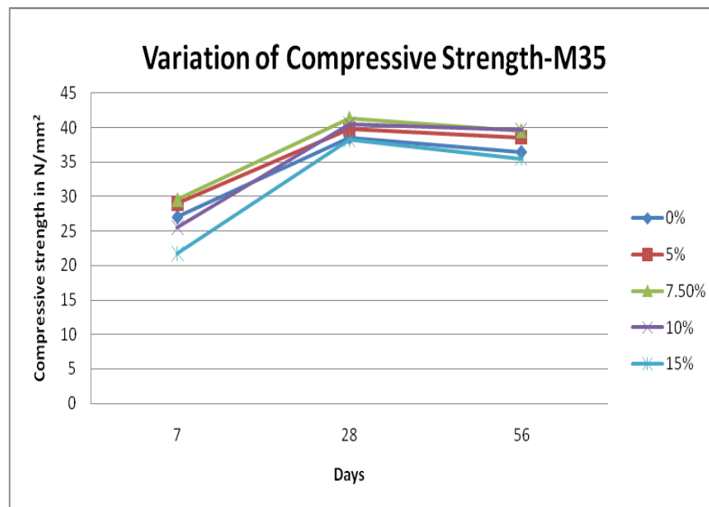
Compressive strengths of M35 grade
