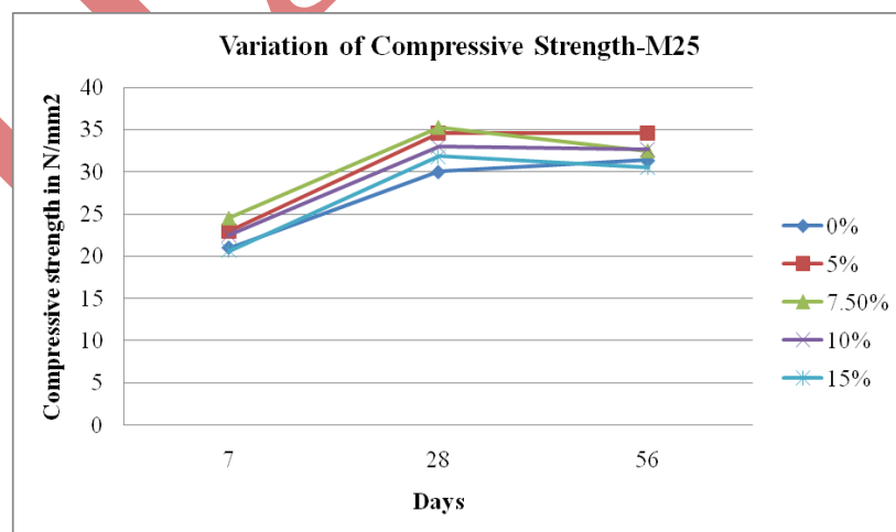
Compressive strengths of M25 grade
