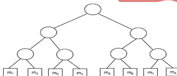
(a) HS-Tree.
