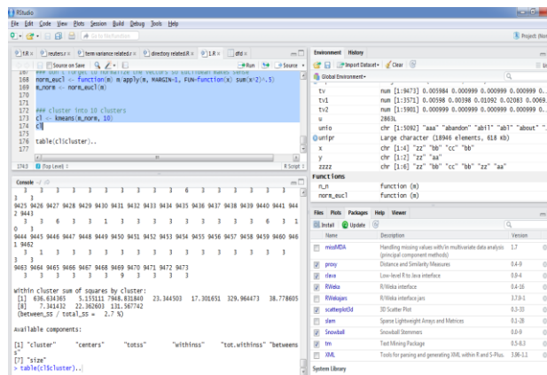
Fig5: K-Means Clustering
