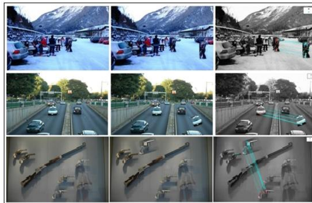
Figure 3:- Results of Hybrid DCT plus SIFT on Some Forged Images of Dataset MICC-F220.
