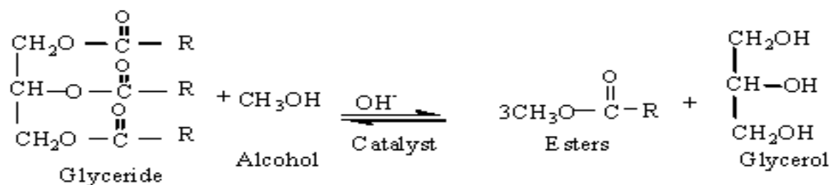
Fig. 1: Transesterification Reaction
