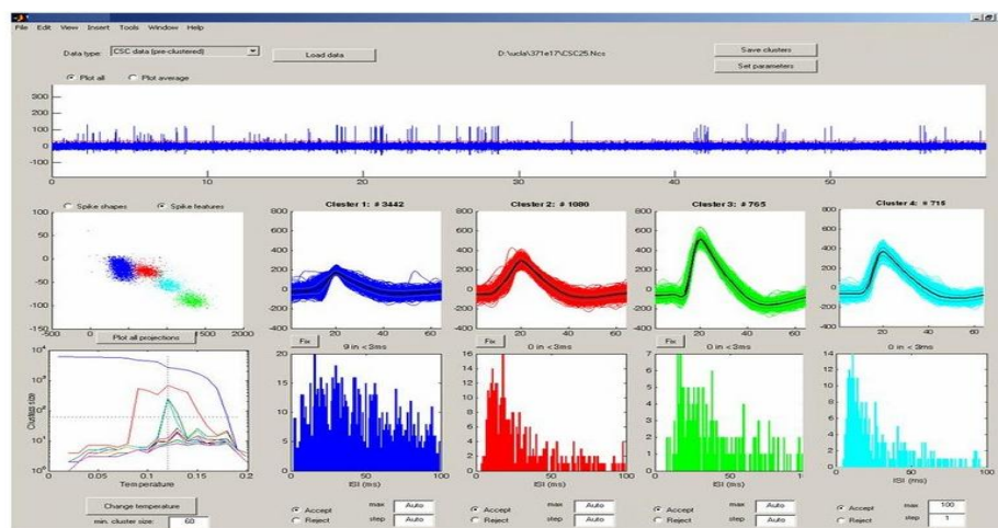
Figure 3. Spike Sorting of a Recording from the Human Medial Temporal Lobe
