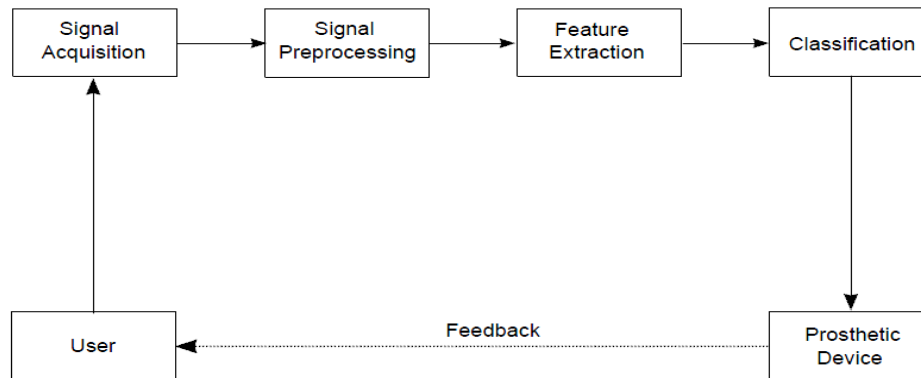
Figure 1: Block Diagram of a BCI System.
