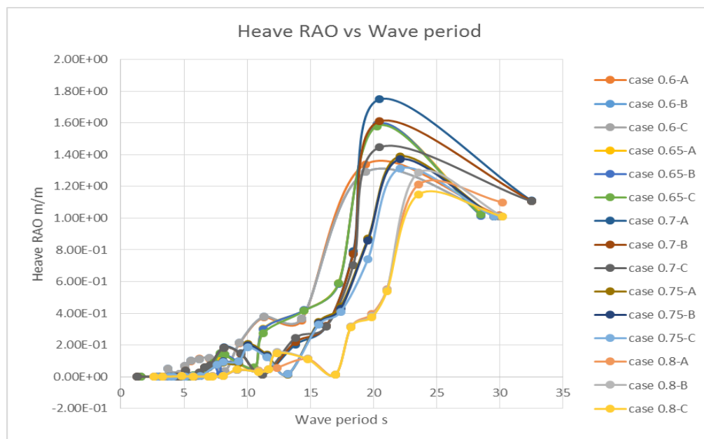
Figure 7. Heave RAO for all Cases of Different Volume Fraction
