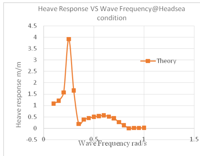
Figure 2: Heave RAO Semisubmersible Hull –Theoretical Calculation
