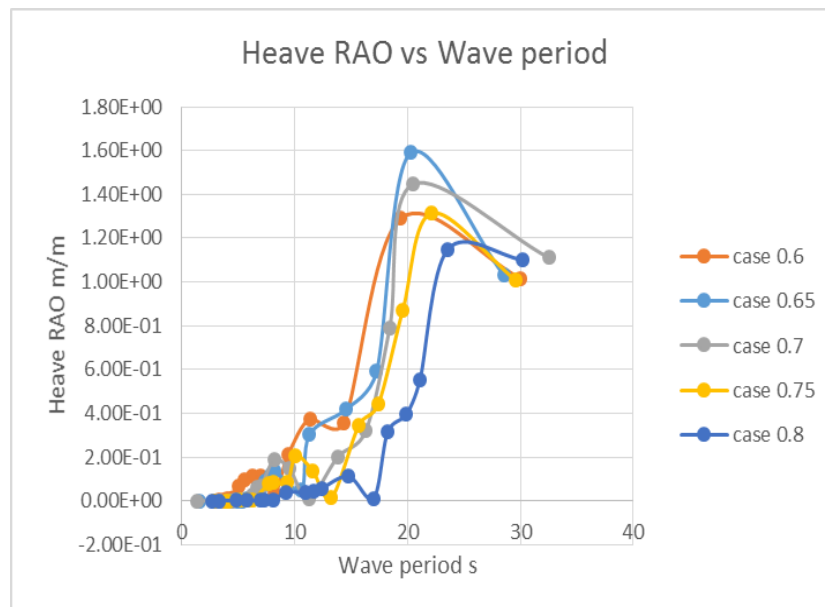
Figure 8 Heave RAO for Different Volume Fraction
