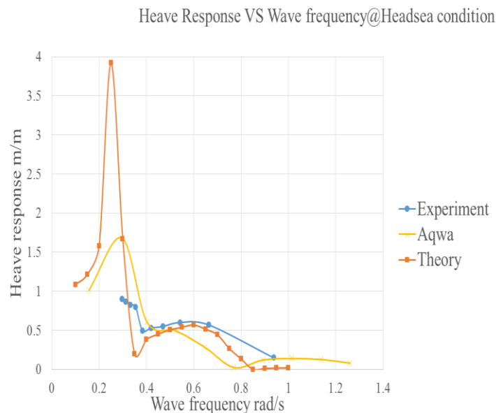
Figure 6: Heave RAO Comparison for GVA 4000
