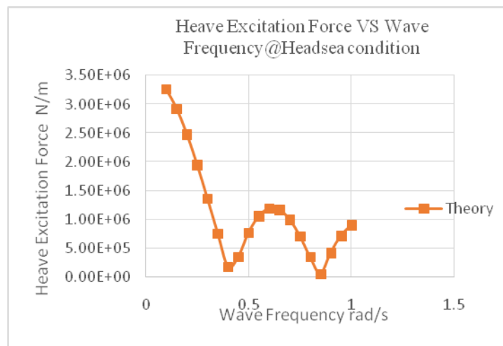
Figure 1: Heave Excitation Force Semisubmersible Hull
