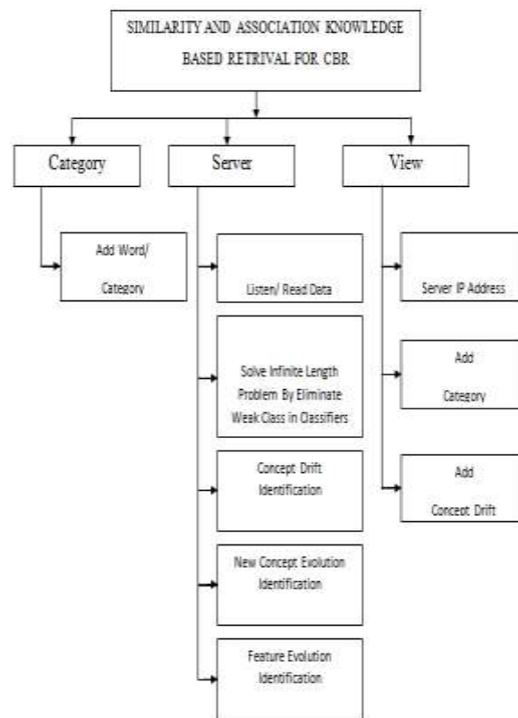
Fig 3.1 Architecture Diagram
