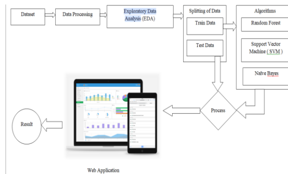
Fig.3: System Architecture
