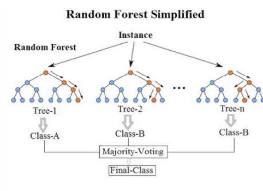
Fig.4: Random Forest
