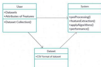
Fig.7: Class Diagram
