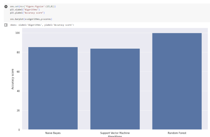
Fig.9: Algorithm Accuracy Score
