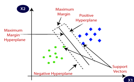
Fig.5: SVM
