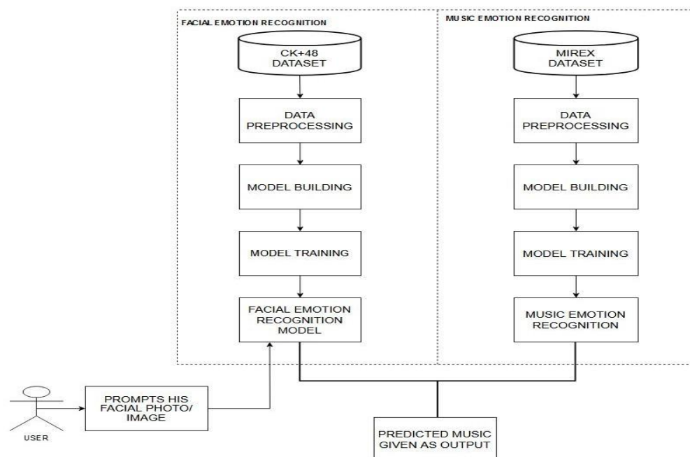
Fig. 1: Model Architecture
