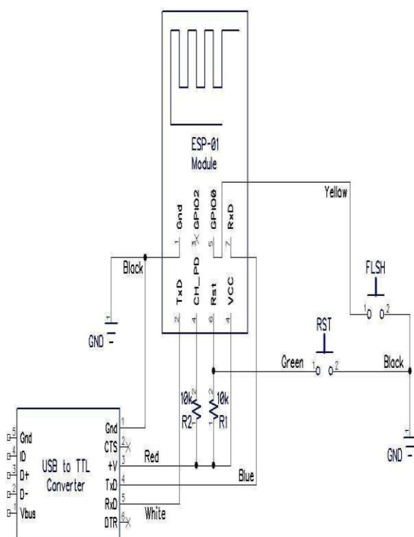
ESP-01 Connection Diagram
