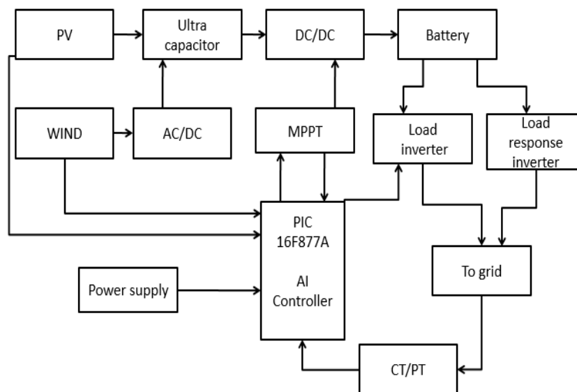
Figure 1 – Block Diagram
