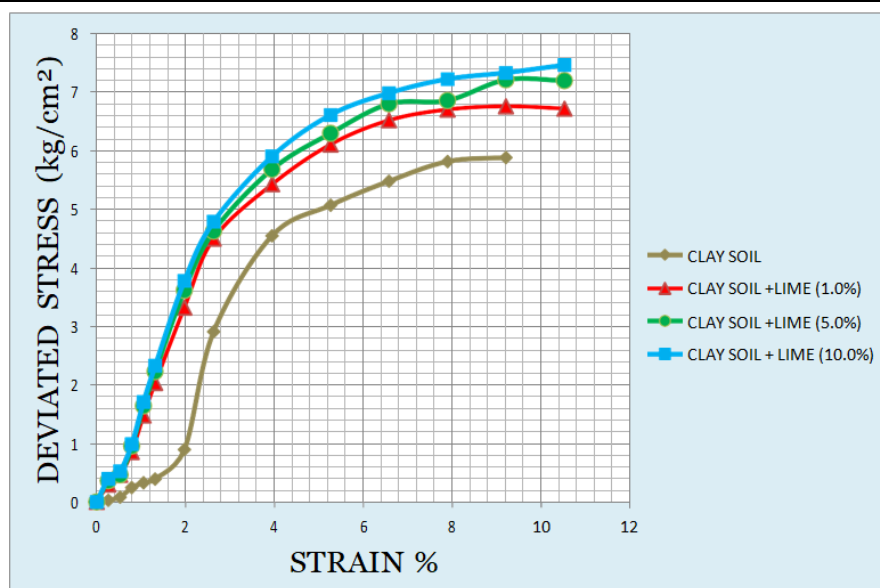
Fig. 7 Variation of shear strength with various proportion of lime.
