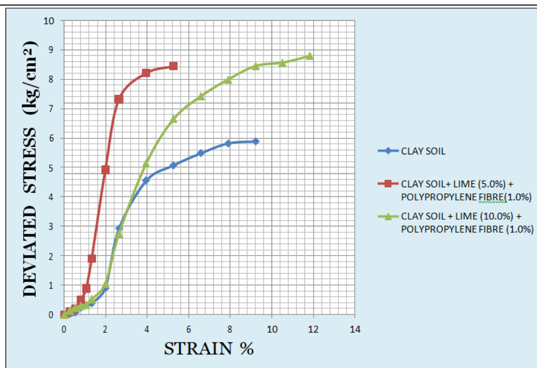
Fig. 8 Variation of shear strength with combination of lime and fiber.
