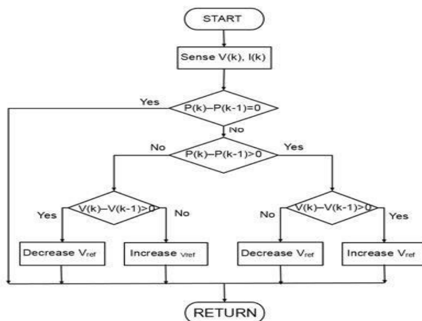
Fig. 2: Flow chart of our project
