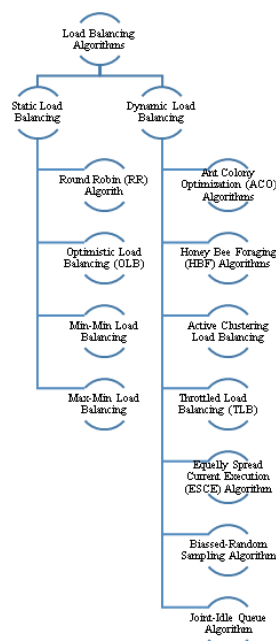
Figure 1: Classification of load balancing algorithms.
