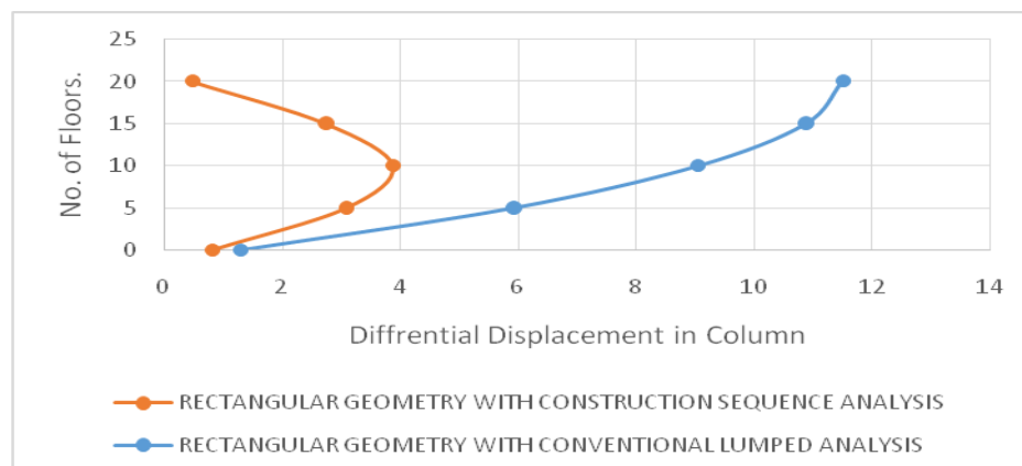
Fig.5.7. Differential Displacement in Column.
