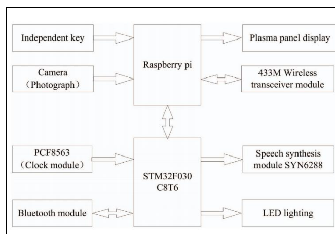
Fig 2.1:Block Diagram of System used in [3]
