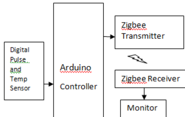
Fig 1. Block Diagram
