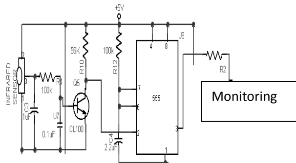
Fig 2. Pulse rate Detection Circuit
