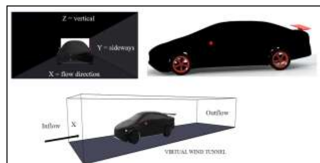
Fig 3.2 Virtual wind tunnel with boundary condition
