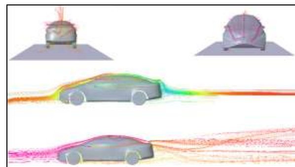
Fig 3.4 Velocity streamline for tubercle & comb (barn) spoiler
