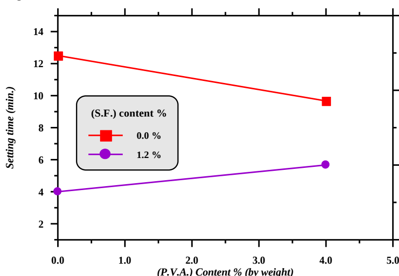
Figure (5) and Table (5): Effect of (P.V.A.) on Setting Time of Local Gypsum Plaster with Various (S.F.) Contents.
