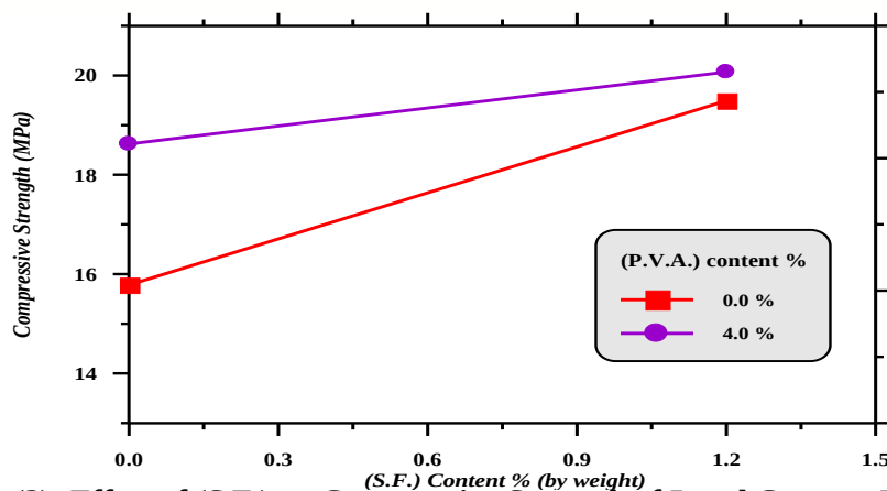
Figure (2): Effect of (S.F.) on Compressive Strength of Local Gypsum Plaster with Various (P.V.A.) Contents
