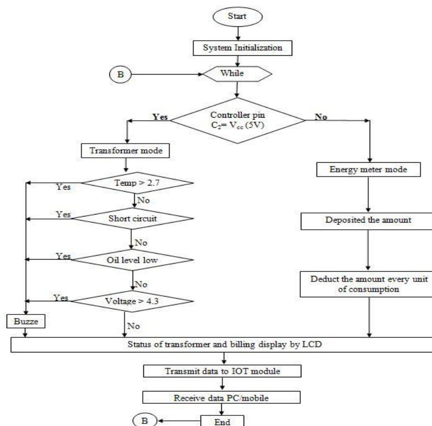
Fig3: Flow chart for health of the transformer and prepaid energy meter
