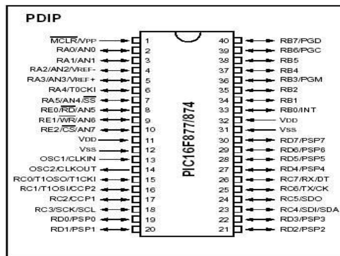
Fig2: pin configuration of pic microcontroller
