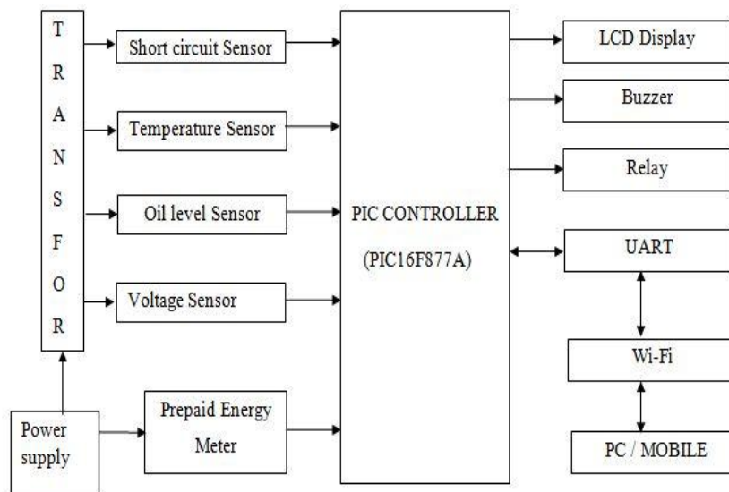
Fig1: block diagram of health of the transformer monitoring with prepaid energy
