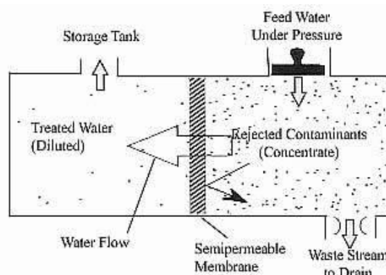
Fig4. RO Filtration
