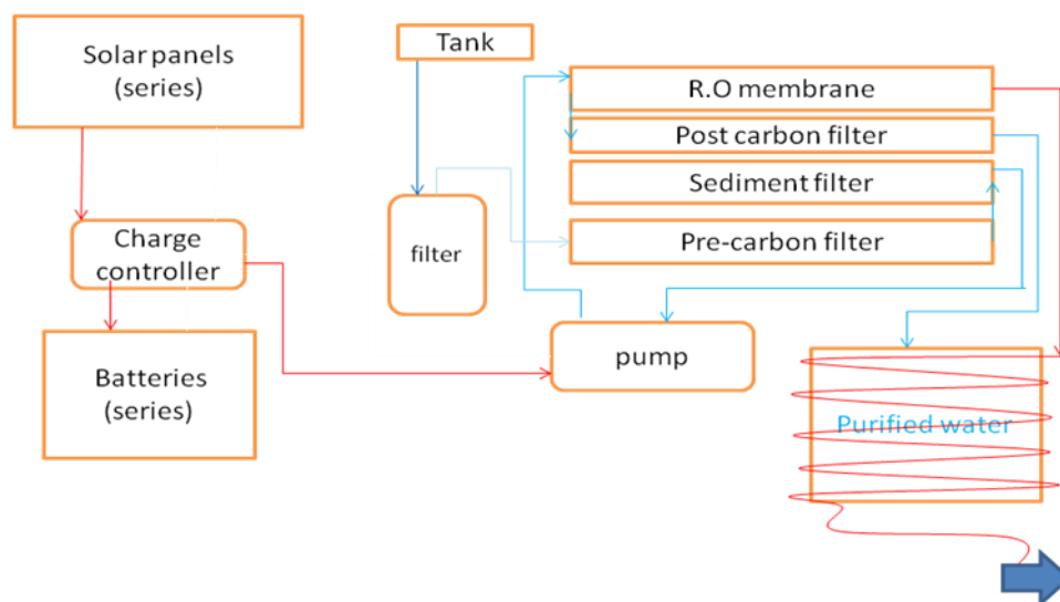
Fig.1 Block Diagram of Purifier unit
