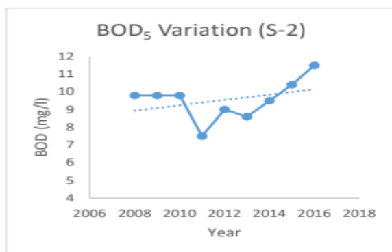
Fig 9. BOD 5 trend analysis
