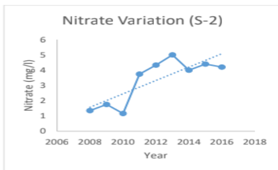
Fig 11. Nitrate trend analysis
