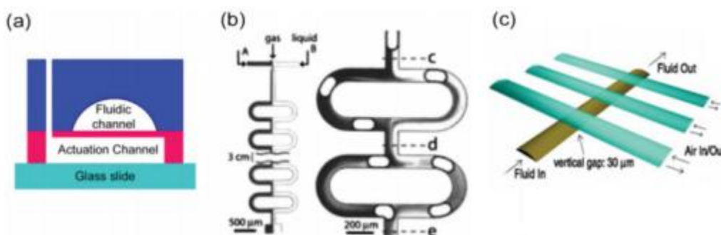
Figure 2: Microfluidic devices; a) a valve, b) a mixer, c) a pump
