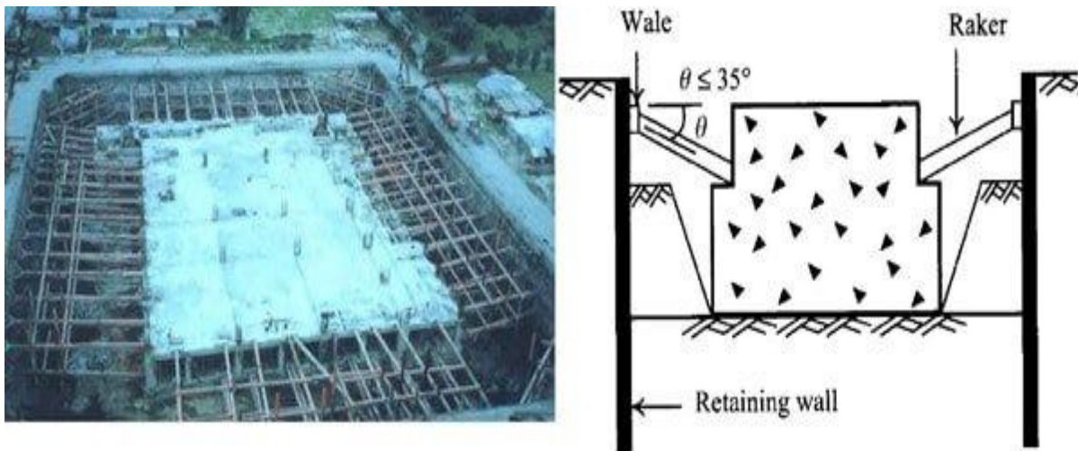
Fig. 6 – Excavation Using Island
