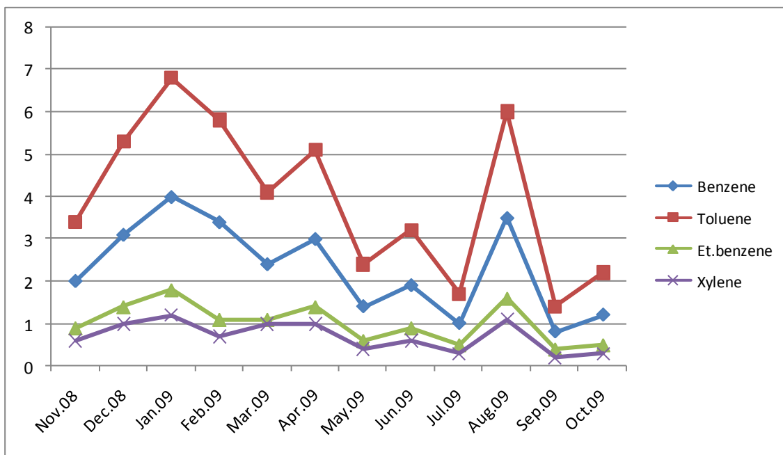
Figure-2 : Monthly mean variation of BTEX ( \mu\text{g}/\text{m}^3 ) at Lashkarpur during Nov.-2008-Oct.-2009.
