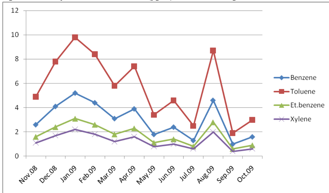
Figure-3 : Monthly mean variation of BTEX ( \mu\text{g}/\text{m}^3 ) at Karbala during Nov.-2008-Oct.-2009.
