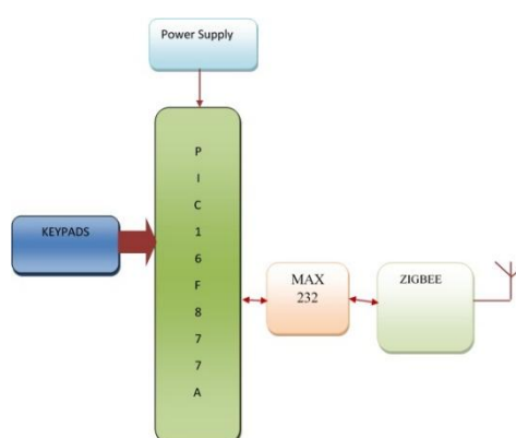
TRANSMITTER
